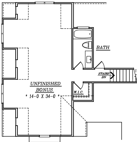
BONUS ROOM PLAN
